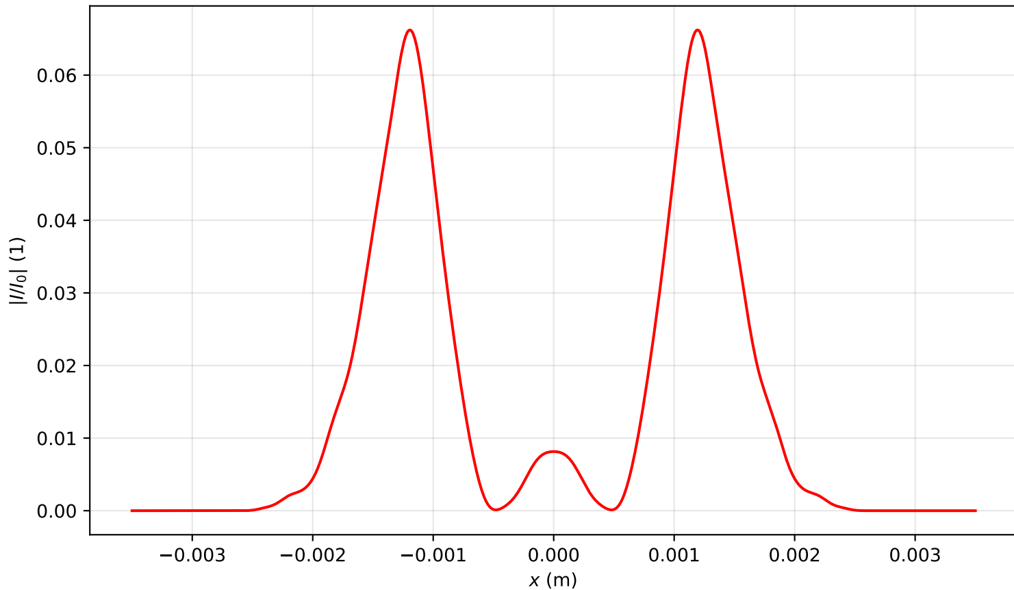
Intensity profile I(x, y = 0, z = 3.582)/I_0 , P_{in}=7.0P_{cr} , artificial time
